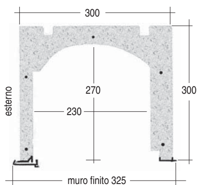
TS BLOCK S 325
