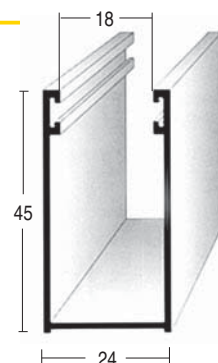
Cod. TS 2445/... 24 x 45 mm
