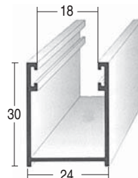
Cod. TS 2430/... 24 x 30 mm
