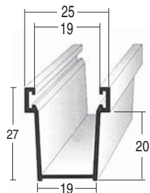
Cod. TS 1927/... 19 x 27 mm
