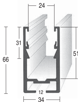
Cod. TS 3466/... 34 x 66 mm
