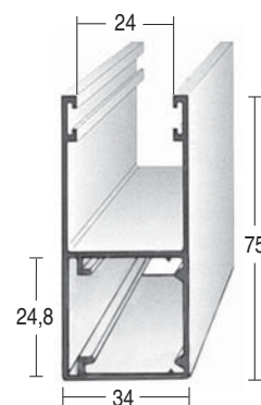
Cod. TS 3475/... 34 x 75 mm
